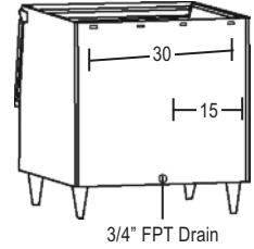
3/4" FPT Drain
