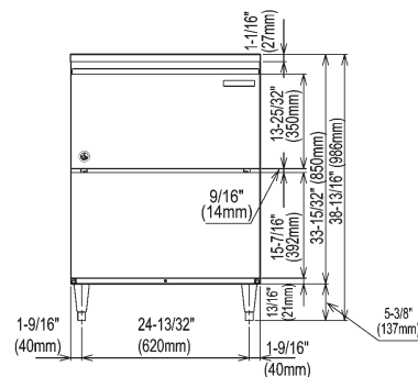
FRONT DIMENSIONS
