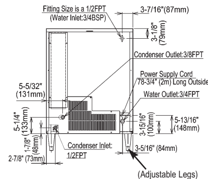
BACK DIMENSIONS
