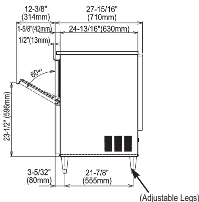
SIDE DIMENSIONS
