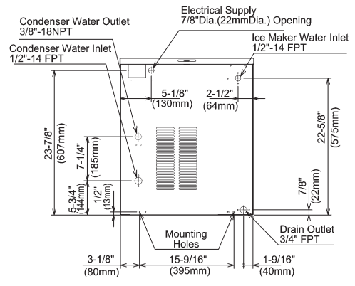
WATER-COOLED UNIT
