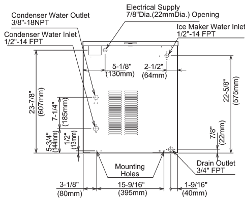
WATER-COOLED UNIT
