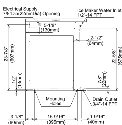
AIR-COOLED UNIT
