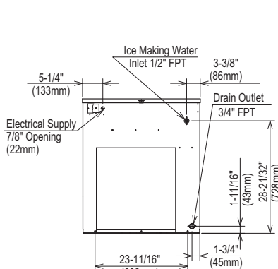
AIR-COOLED UNIT
